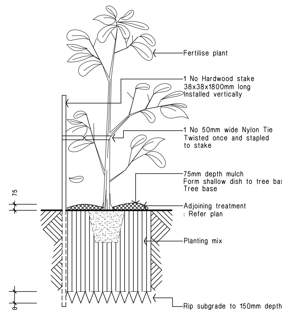
45 litre Tree planting Detail. Not To Scale.
